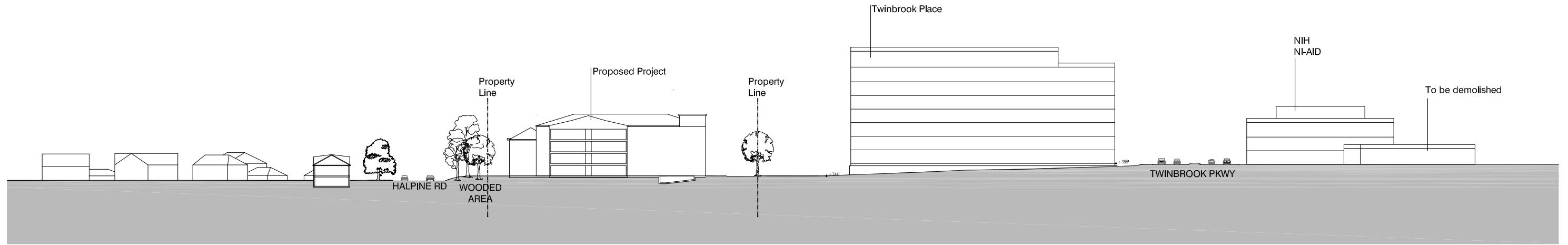
1 NORTH-SOUTH SECTION
