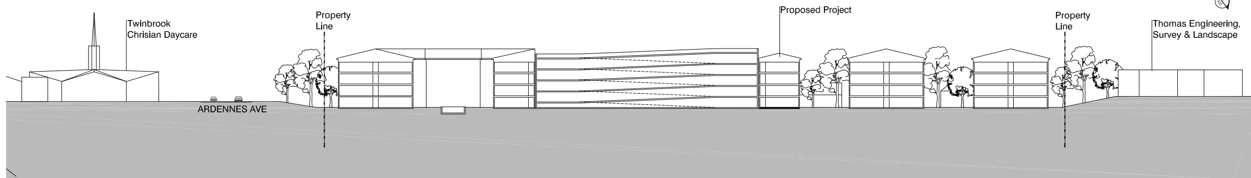
3 EAST-WEST SECTION
